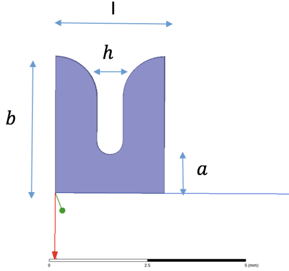
Figure 22: cavity shape of the TW 2\pi/3 mode
