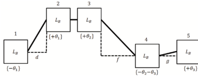
Figure 12: Diagram of a five-bend chicane [16]. Not to scale.
