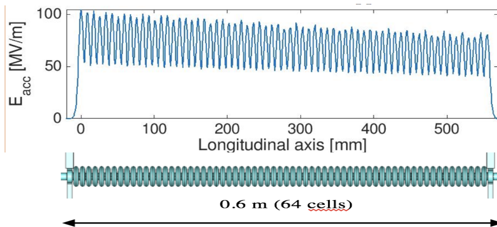
Figure 19: Accelerating field as a function of longitudinal axis.
