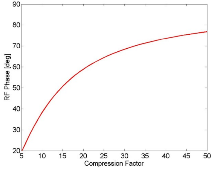
Figure 8: RF phase of injector linac vs. linear compression factor at the first chicane, for assumed value of 0.1 deg rms phase jitter and specified 1% rms bunch length jitter. The accelerating phase is at 90 deg. The compression scheme discussed above suggests a linac phase not exceeding 60 deg (30 deg from the crest).
